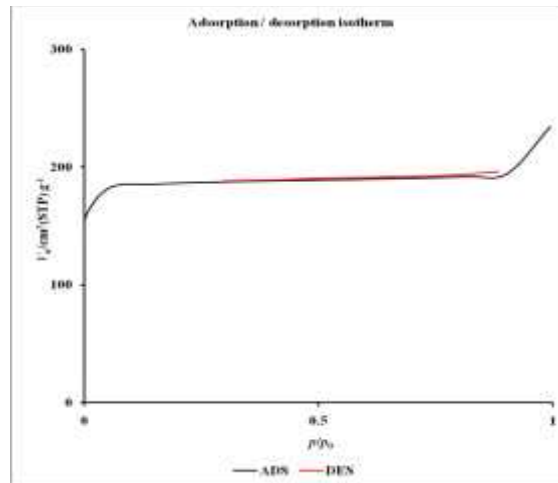
Figure 5. N_2 adsorption- desorption isotherm.
