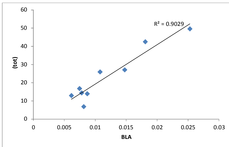
Figure 8. The first static hyperpolarizability ( \chi_{tot} ) versus BLA for all substituents, except X= \text{NH}_3^+ , CN, \text{NO}_2 , COOH.
