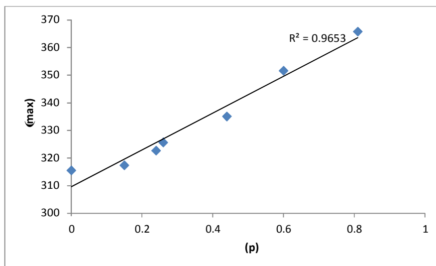
Figure 3. Maximum Absorption wavelength ( \lambda_{\max} ) versus Hammett constants ( \rho ) (except for Me, OH, \text{NH}_2 , CN).
