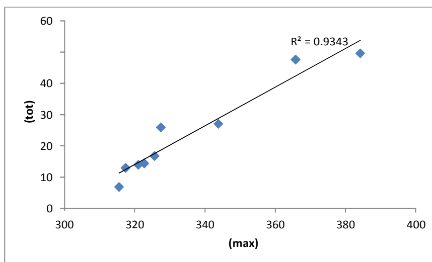
Figure 7. The first static hyperpolarizability ( \chi_{tot} ) versus \chi_{max} for all substituents, except X= \text{NH}_2 , \text{NH}_3^+ , CN.
