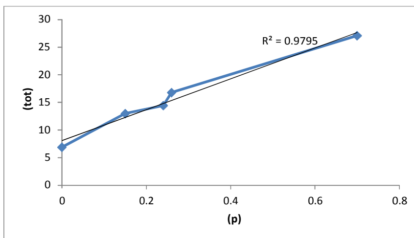
Figure 6. The first static hyperpolarizability ( \chi_{tot} ) versus \rho for X= H, F, Cl, Br, CN.
