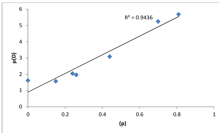
Figure 2. Dipole moment ( \mu ) versus \rho Hammett constants ( \rho ) (except for \text{NH}_3^+ that induces a very large dipole moment of 18 D not reflected by its \rho value of 0.6). The line has a linear correlation coefficient of R^2 0.94.
