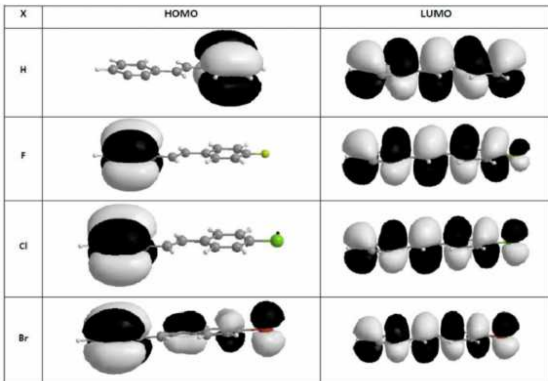
Figure 4. Frontier orbitals energies versus Hammett constants ( \rho ) (except for \text{NH}_3^+ ).
